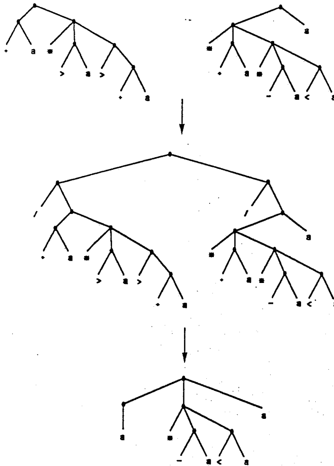
FIGURE 2 Interaction between functions. Two algorithmic strings (top) represented as trees interact by forming a new algorithmic string (middle) that corresponds to a function composition. The new root with its two branches and ' operators is the algorithmic notation for composing the functions. The action of the unary ' operator ("quote"-operator) consists in preventing the evaluation of its argument. The interaction expression is evaluated according to the semantics of the language and produces an expression (bottom) that represents a new function.
