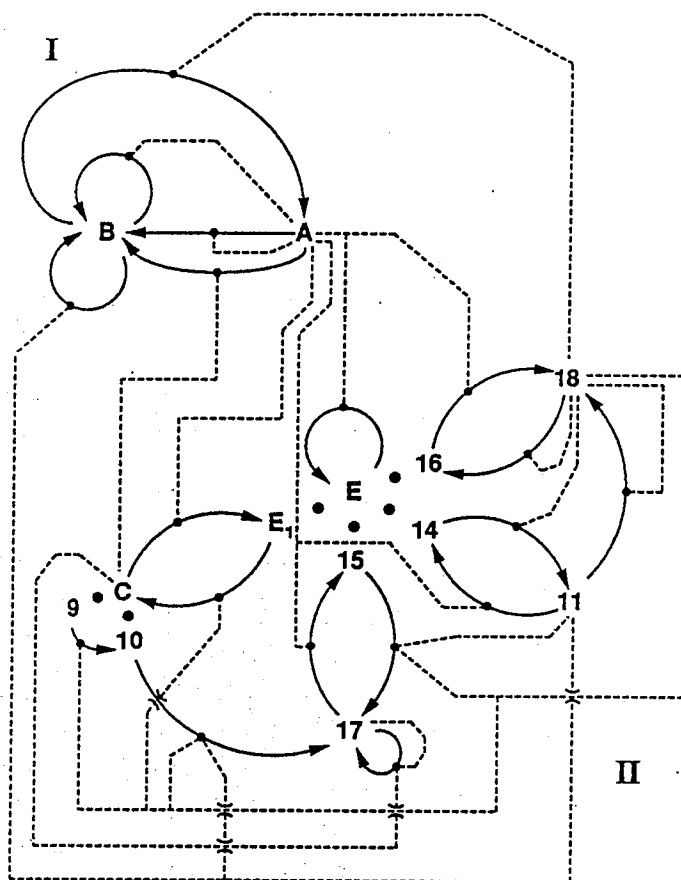
FIGURE 4 Interaction graph of a metastable Turing gas transient. The interaction graph of the functions present in the system after 3 \times 10^5 collisions is shown. The system started with 1000 random functions, and conserves the total number of particles (1000). The numbers denote the individual functions according to their lexicographic ordering (not shown). Capital letters denote sets, where A = \{1, 2, 3, 4\} , B = \{5, 6, 7, 8\} , C = \{9, 10\} , E = \{12, 13, 14, 15, 16\} , and E_1 = \{12, 13\} \in E . Solid arrows indicate transformations and dotted lines functional couplings. A dotted line originates in a function, say k , and connects (filled circle) to a solid arrow, whose head is j and whose tail is i . This is to be interpreted as j = k(i) . Large filled circles indicate membership in a particular set. Function 17 is an identity function. Note: all dotted lines and solid arrows that result from 17 copying everything else in addition to itself have been omitted. The function set is closed with respect to interaction.
