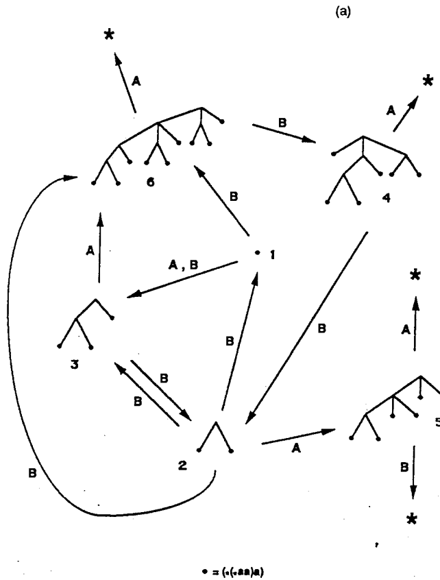
FIGURE 5 (a) Interaction graph of a metastable Turing gas state without copy reactions. The figures show the interaction pathways among two polymer families established after 5 \times 10^5 collisions starting from random initial conditions. The tree structure of the functions is displayed. The leaves are "monomers" representing the functional group indicated at the bottom of each graph. Solid arrows indicate transformations operated by function(s) belonging to the family denoted by the arrow label(s). Stars in the transformation pathways represent functions that were not present in the system at the time of the snapshot ("innovative reactions"). Due to the polymeric architecture of the functions, the system remains highly innovative. There are always (at least) two functions in the system that a polymerizing function (like the monomer 1 in 5(a)) can combine in order to produce a third one not in the system. The "space limit" tag.
