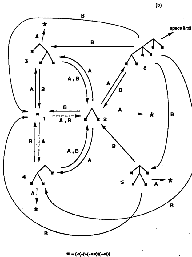
FIGURE 5 (continued.) (b) indicates that the corresponding reaction product would hit the length limitation imposed on each individual function expression (300 characters in the present case).
