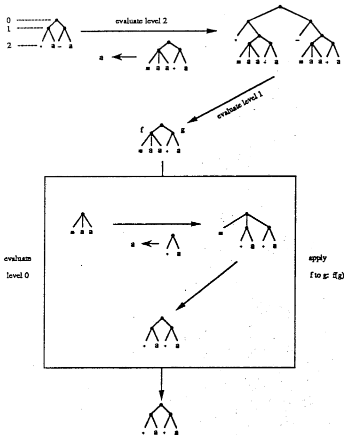
FIGURE 1 Evaluation example. The value of the expression ((+a)(-a)) is computed when the variable a takes on the value ((*aa)(+a)) . The interpretation process follows the tree structure until it reaches an atom (leaf). In this case it happens at depth 2. The atoms are evaluated: the operators “+” and “-” remain unchanged, while the value of a is given by ((*aa)(+a)) . The interpreter backs up to compute the values of the nodes at the next higher level using the values of their children. The value of the left node at depth 1 is obtained by applying the unary “+”-operator to its sibling (which has been evaluated in the previous step). The “+” operation returns the first subtree of the argument, (*aa) in this case. Similarly, the value at the right depth 1 node is obtained by applying the unary “-”-operator to its argument ((*aa)(+a)) . The “-” operation deletes the first subtree of its argument returning the remainder, (+a) . The interpreter has now to assign a value to the top node. The left child’s value is an expression representing again a function. This function, (*aa) , is labelled as f in the figure. Its argument is the right neighbor sibling, (+a) , labelled as g . Evaluating the top node means applying f to g . This is done by evaluating f while assigning to its variable a the value g . The procedure then recurs along a similar path as above, shown in the box. The result of f(g) is the expression ((+a)(+a)) . This is the value of the root (level 0) of the original expression tree, and therefore the value of the whole expression, given the initial assignment. The example can be interpreted as “function ((+a)(-a)) applied to function ((*aa)(+a)) ”.
