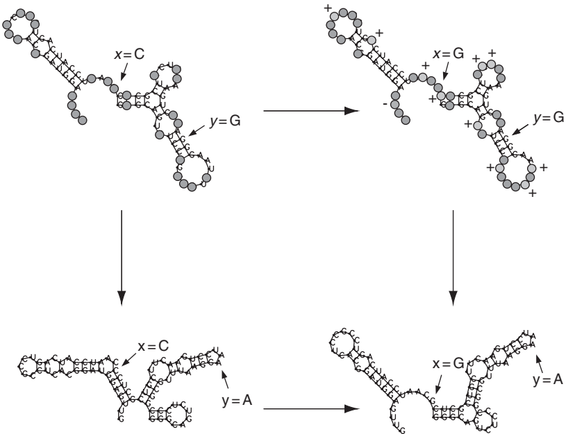
Figure 5.3 Epistasis*
