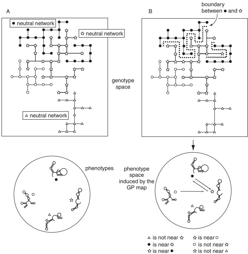
Figure 5.5 Neutral networks and shape space topology.
